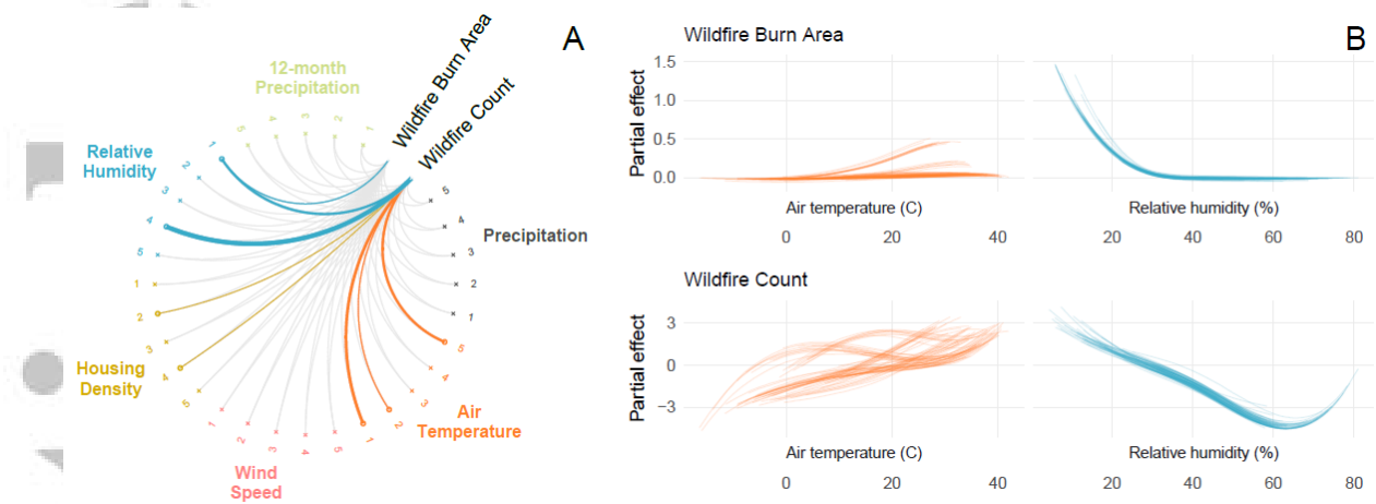
Figure 5: Bayesian approaches can reduce the complexity of interactive drivers. Joseph et al. (2019) used B-splines to predict wildfire burn area and count by month. Using 6 predictor variables with 5 basis vectors each (to account for nonlinear effects), the chord diagram (left panel) shows that only 8 out of the 60 global coefficients were significant at the 95% credible level (colored lines). Line width is scaled by the magnitude of the coefficient, indicating a stronger effect. When spatial interactions were accounted for using nested Level 1-3 EPA ecoregions, the resultant 10,416 coefficients reduced to just 18 at the 95% credible level. As examples, the four panels on the right show partial effects of daily maximum air temperature and minimum relative humidity on wildfire burn area and counts, where each line represents the estimated effects for each EPA level 3 ecoregion (adapted from Joseph et al., 2019).
