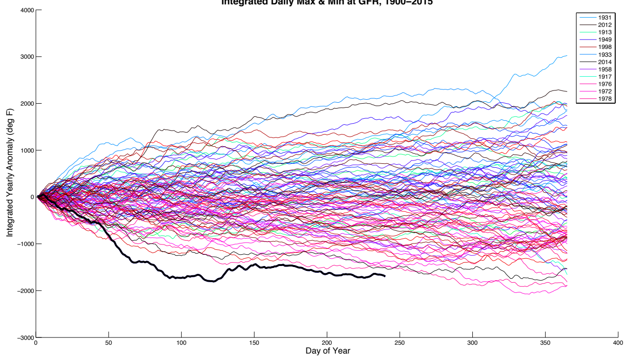
Integrated Daily Max & Min at GFR, 1900–2015
