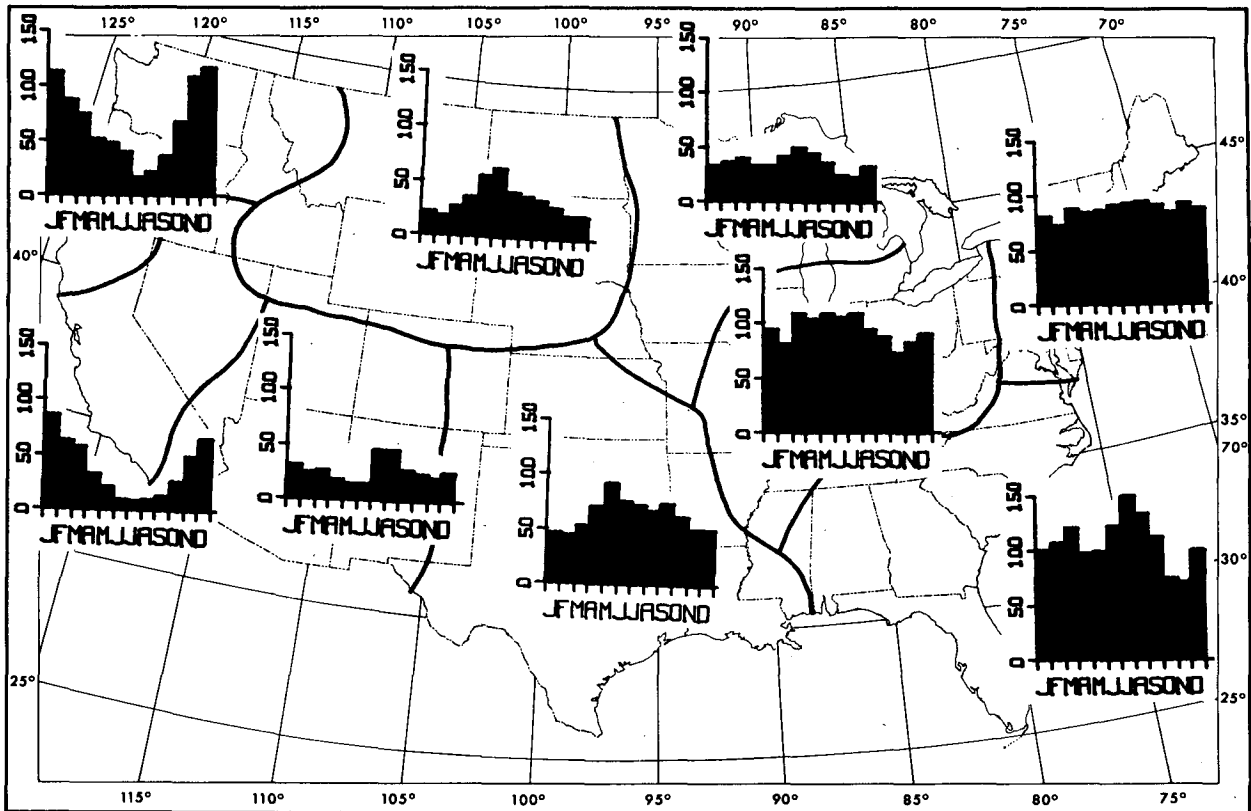
FIG. 3. Mean monthly total precipitation (millimeters) in each of nine regions delineated by a rotated principal component analysis of the PDSI (from Karl and Koscielny, 1982).
